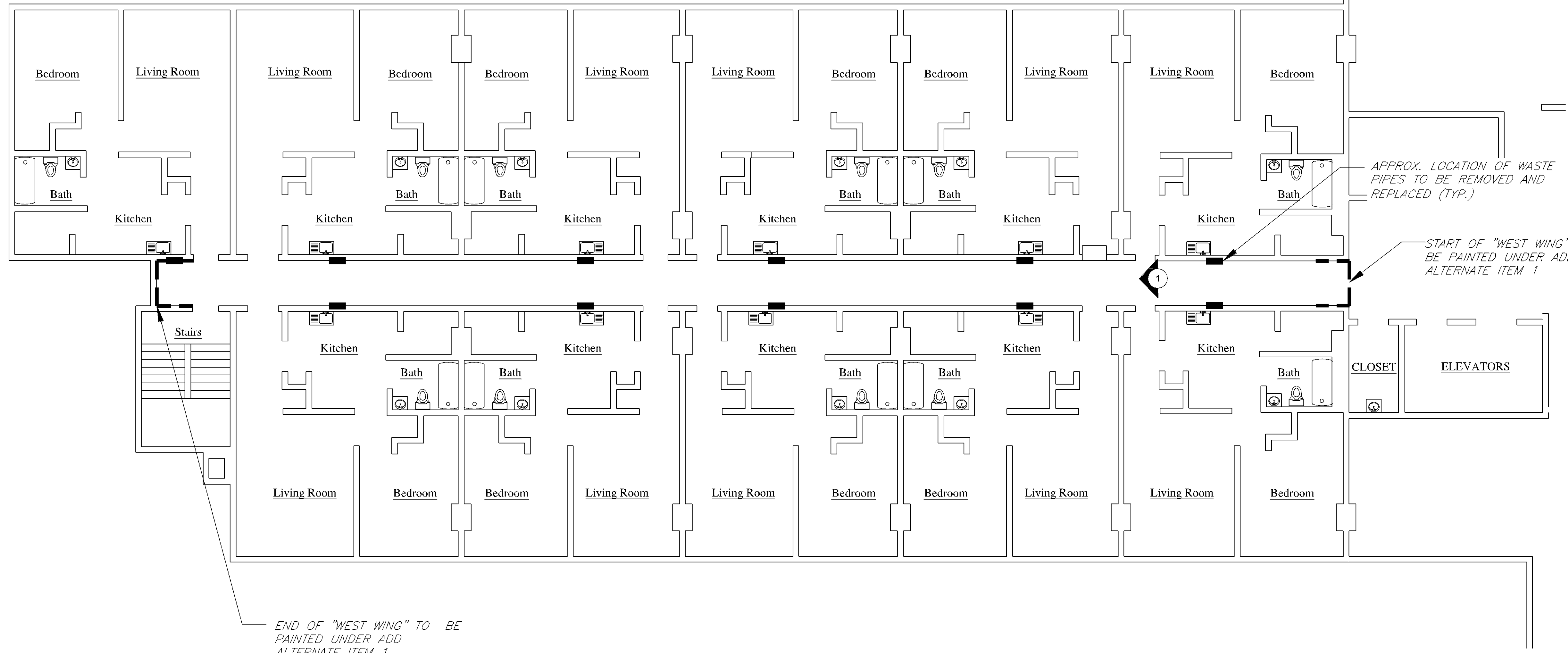
TYPICAL VIEW OF EXISTING PIPE
