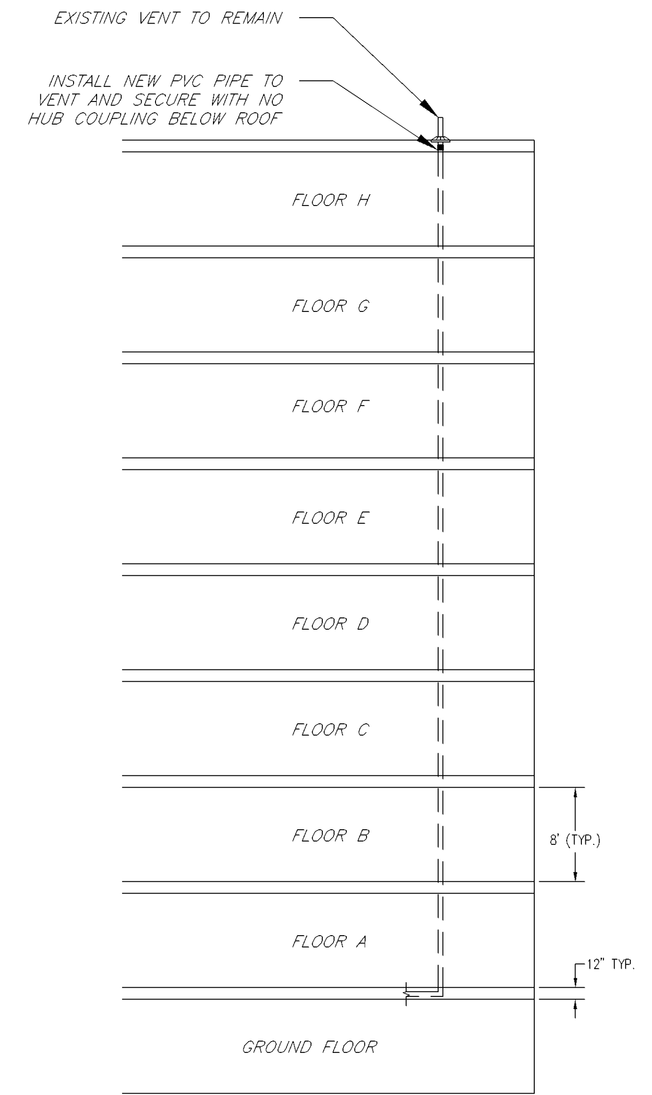
SECTION VIEW OF BUILDING
