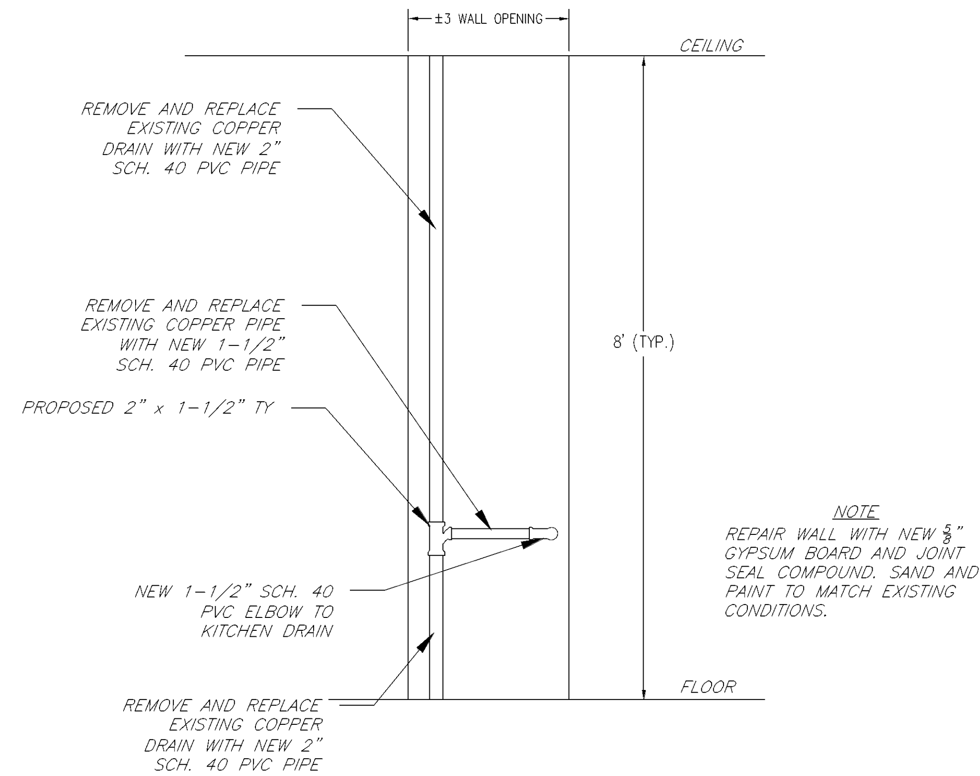
TYP. DRAIN REPAIR
