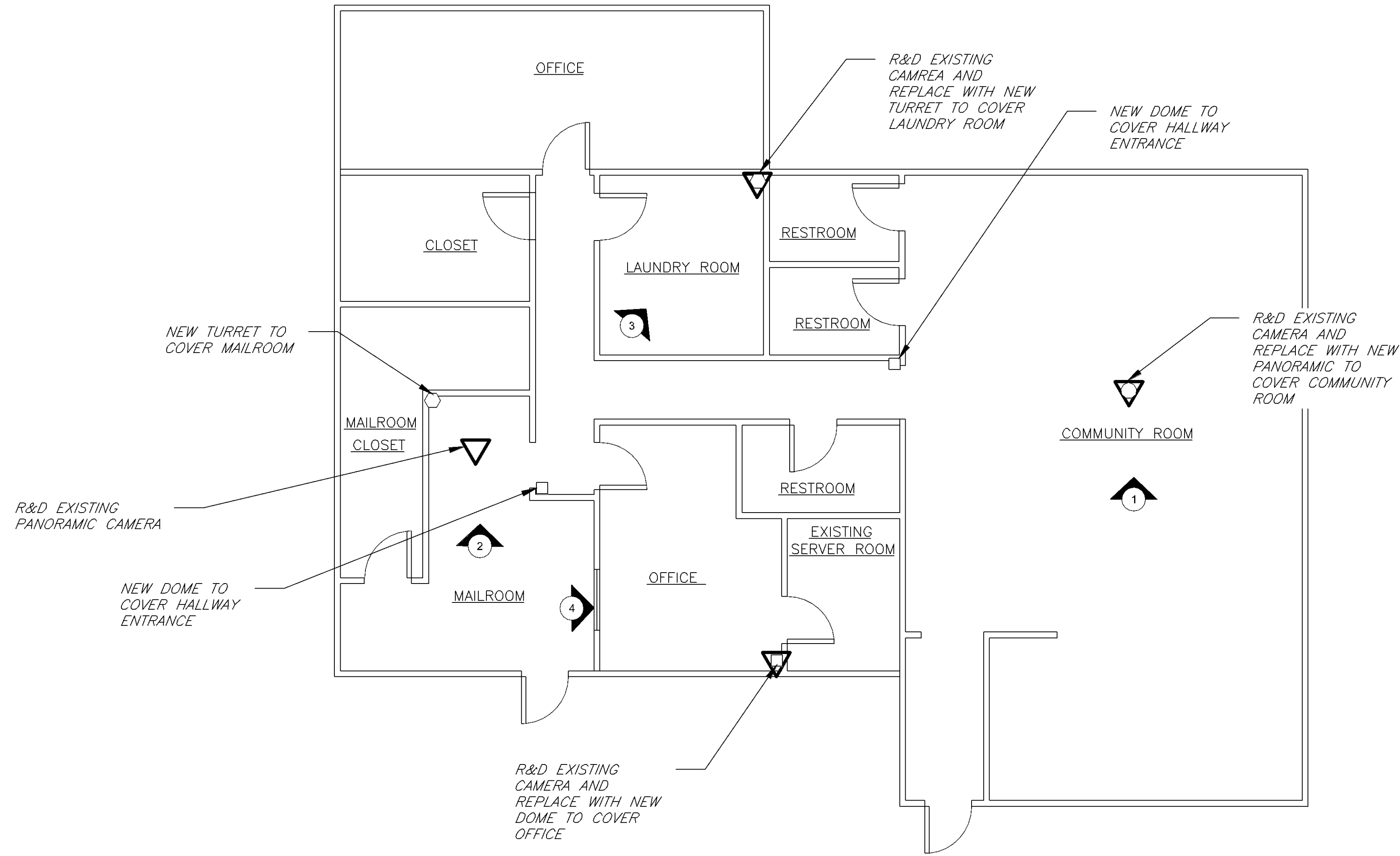
COMMUNITY CENTER NOT TO SCALE
